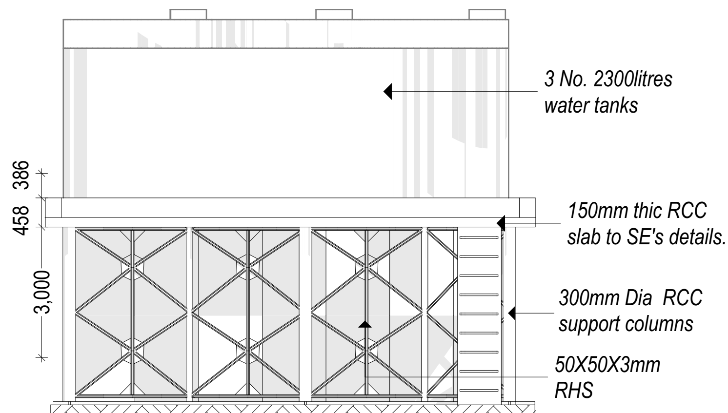
ELEVATED TANK STAND DETAILS
