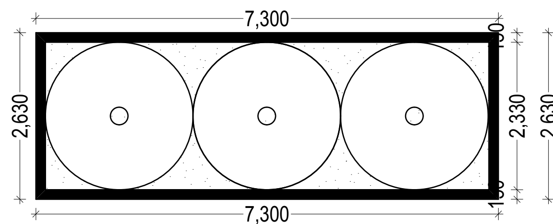
ELEVATED TANK FLOOR PLAN
